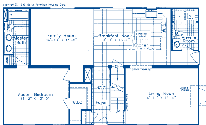
STANDARD BASEMENT PLAN
