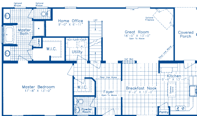
STANDARD BASEMENT PLAN
