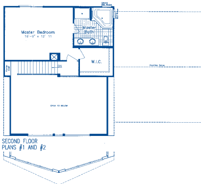
OPTIONAL GABLE PROJECTION w/ PROWL OVERHANG
