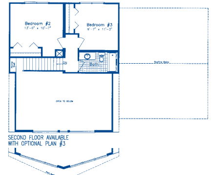
OPTIONAL GABLE PROJECTION w/ PROWL OVERHANG
