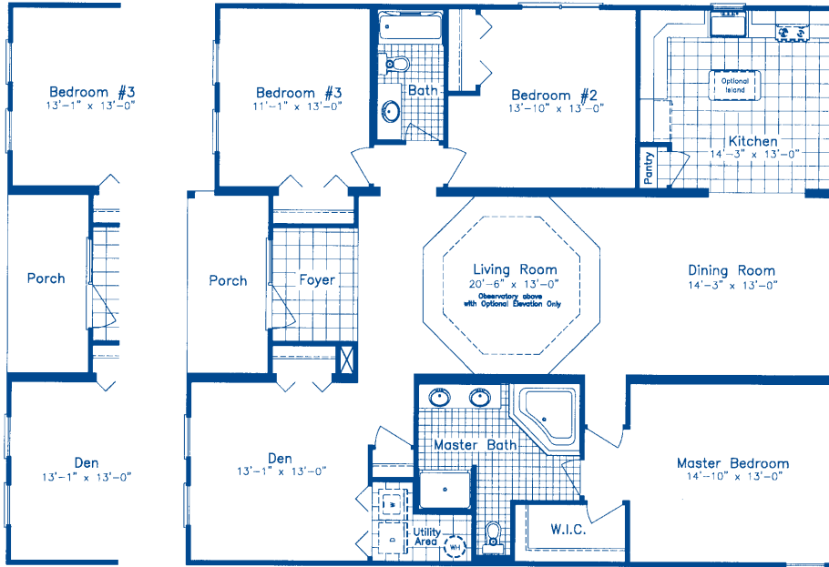
OPTIONAL FRONT PROJECTION
